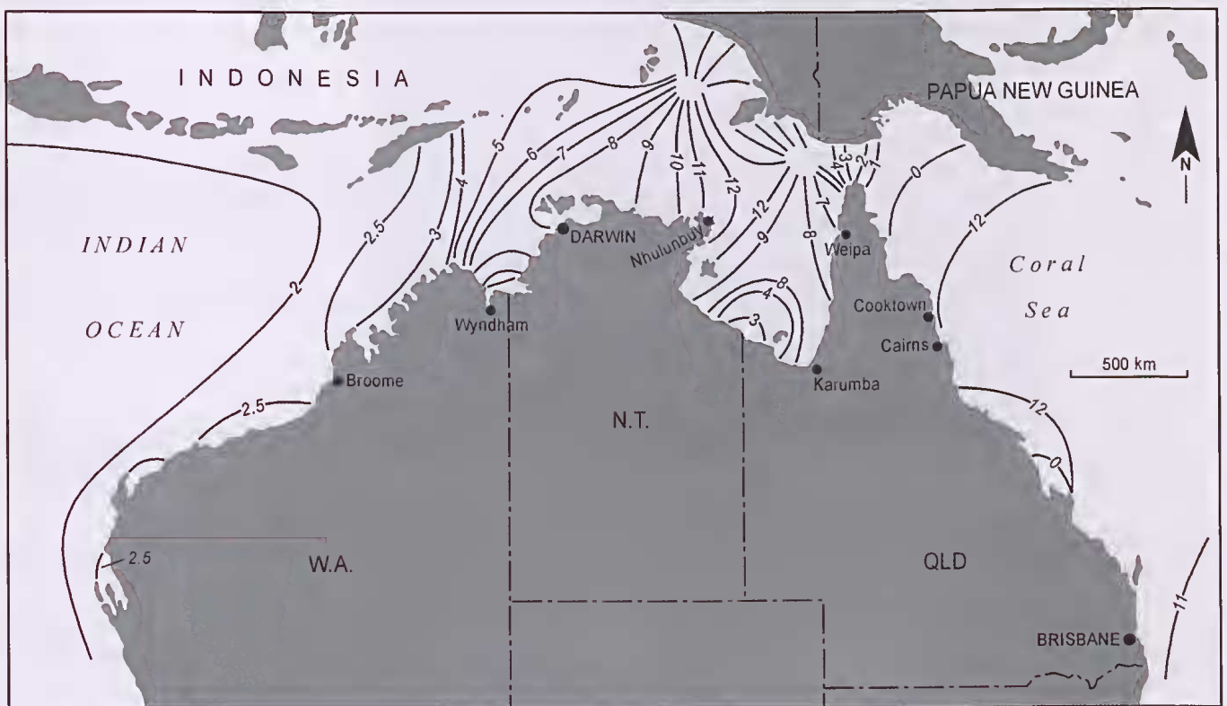
Co-tidal range
